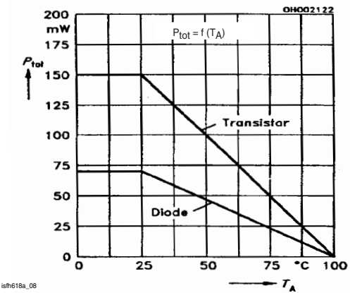
Fig. 10 Permissible Power Dissipation
